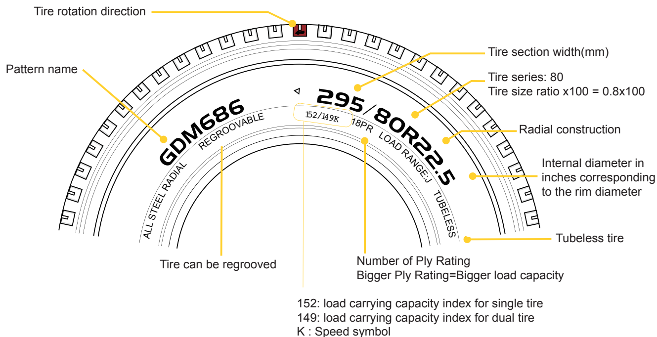
Load Range Chart
